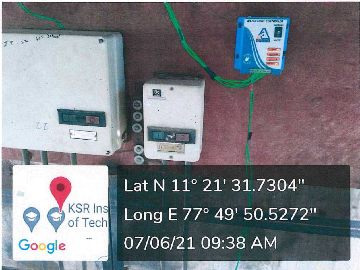
OVERHEAD WATER TANK - WATER LEVEL CONTROLLER
